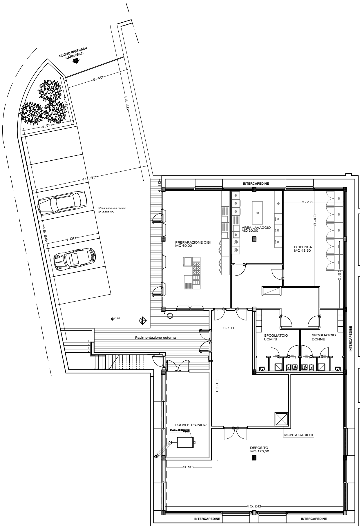
PLANIMETRIA PIANO SEMINTERRATO scala 1:100 POST OPERAM
